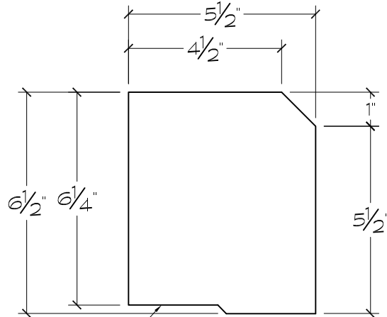
CROSS SECTION
